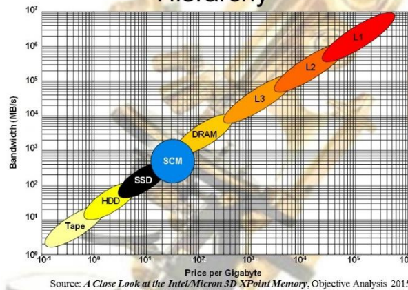
Figure 2. SCM’s Position in the Memory Hierarchy
